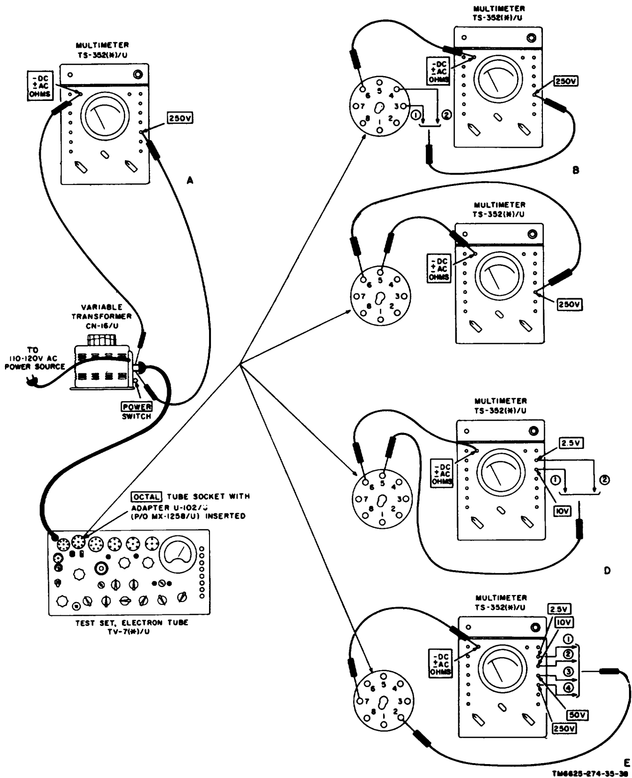
Figure 38. Voltage tests.
