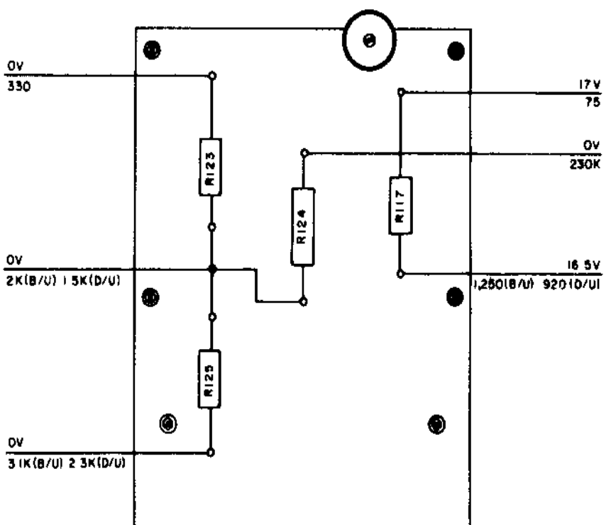
F RESISTOR MOUNTING BOARD TV-7B/U AND TV-7D/U
