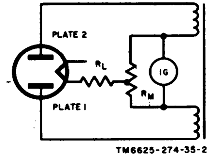
Figure 4. Rectifier diagram.
