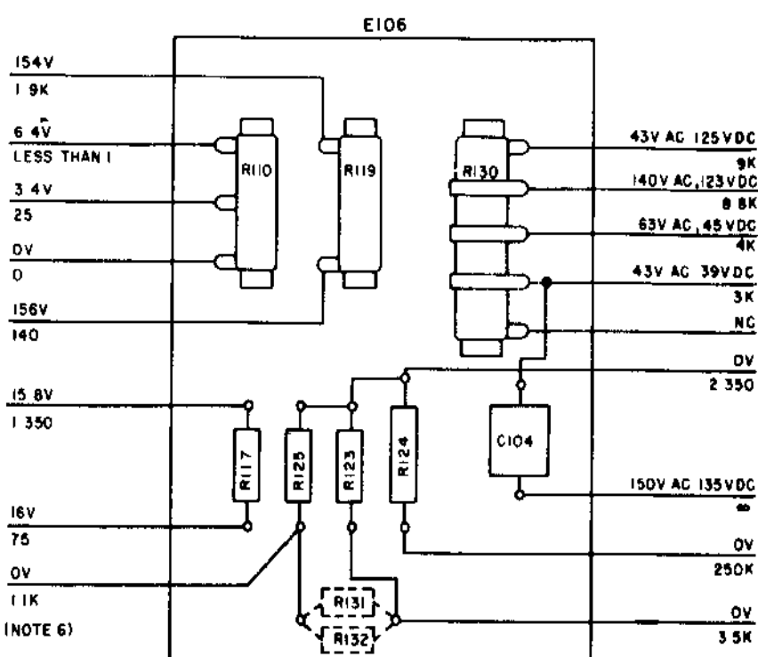
C TV-7A/U SERIAL NUMBERS 1201 THROUGH 9492
