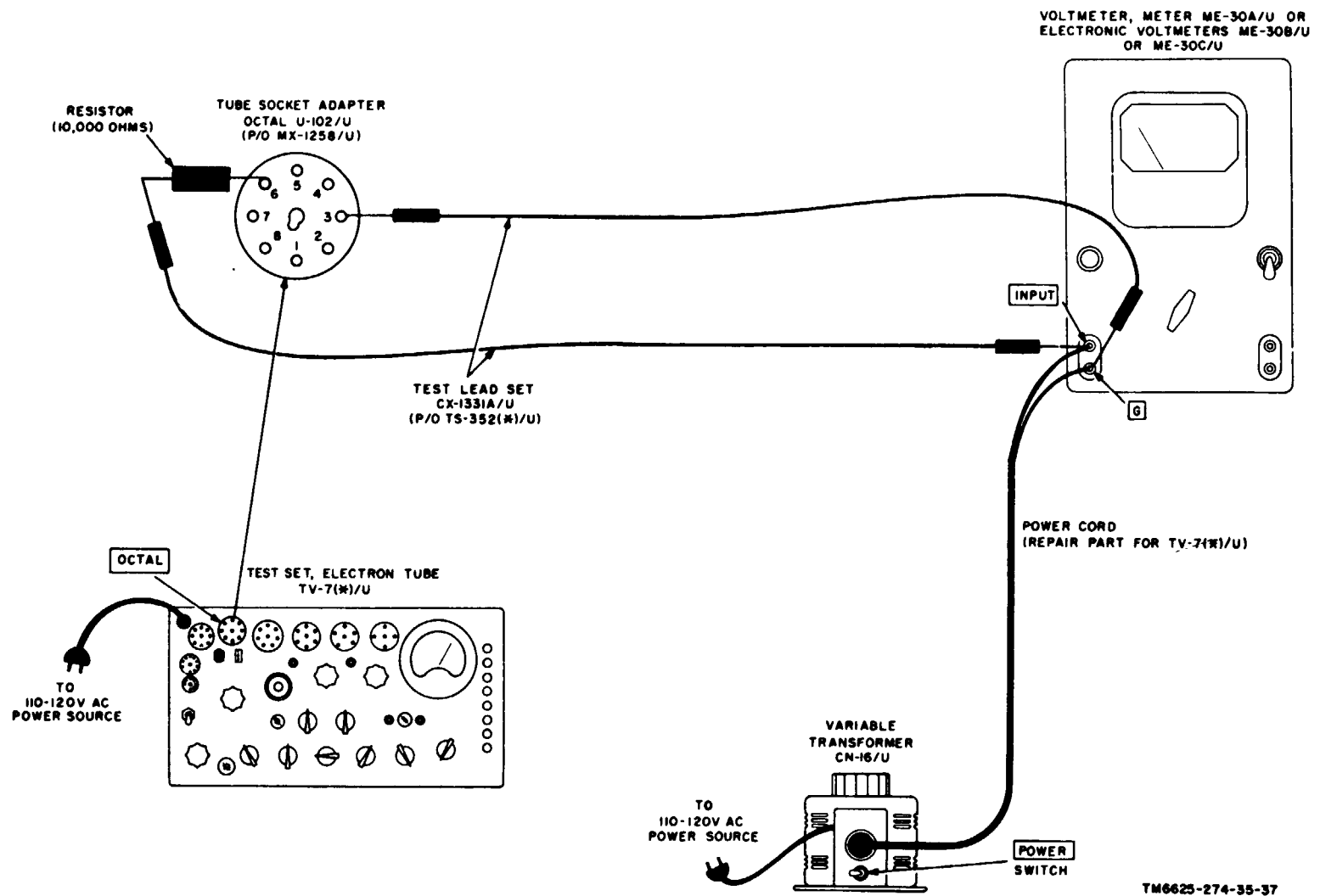
Figure 37. Calibration test.
