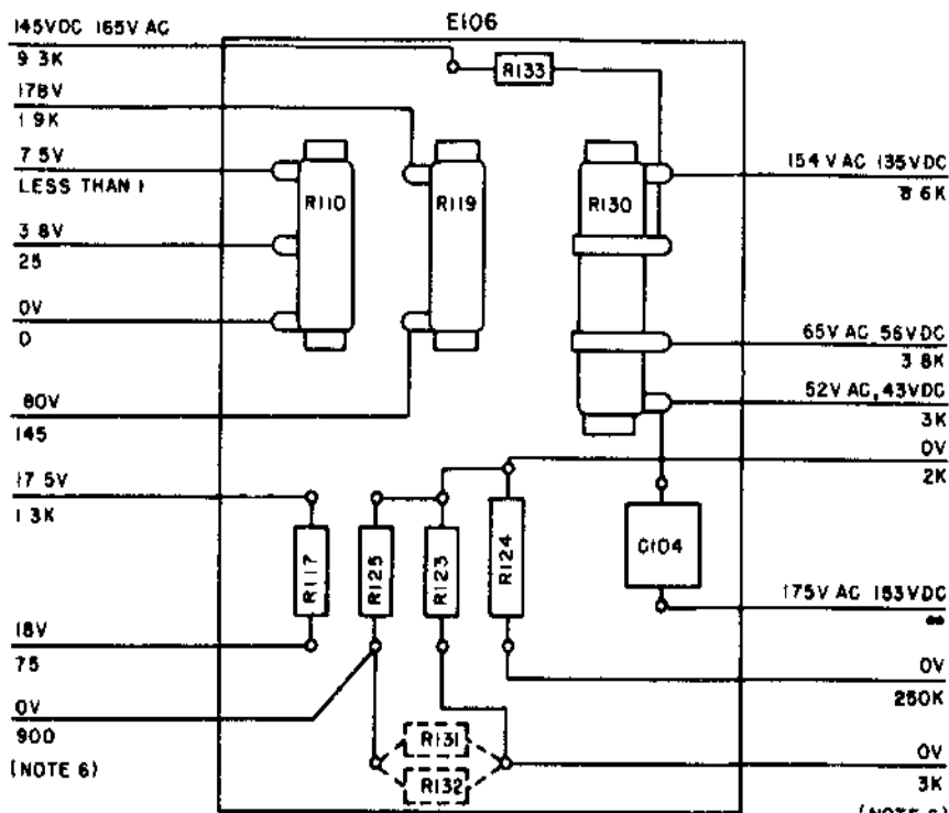
B TV-7A/U SERIAL NUMBERS 1 THROUGH 1200
